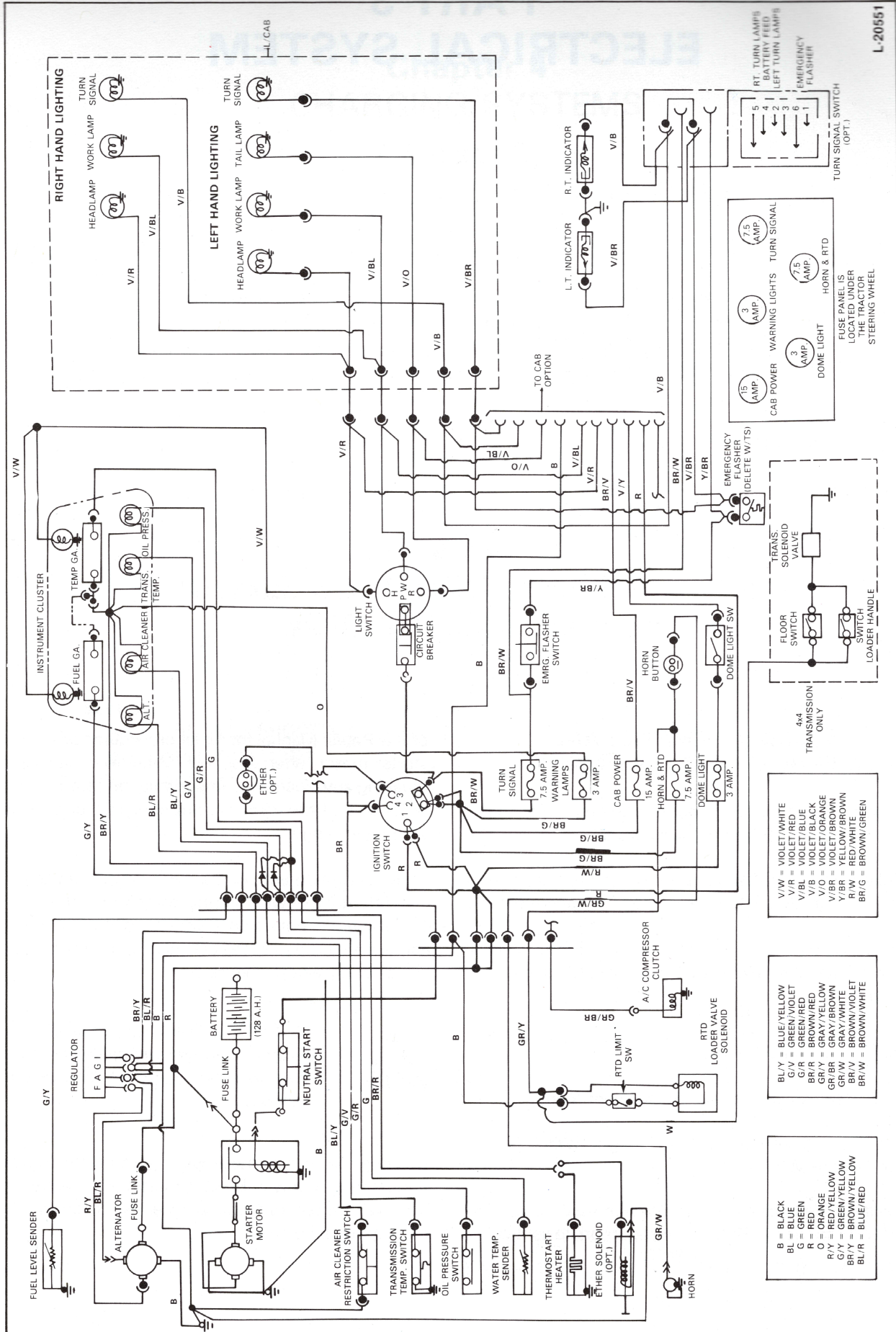
Figure 1 General Wiring Schematic
