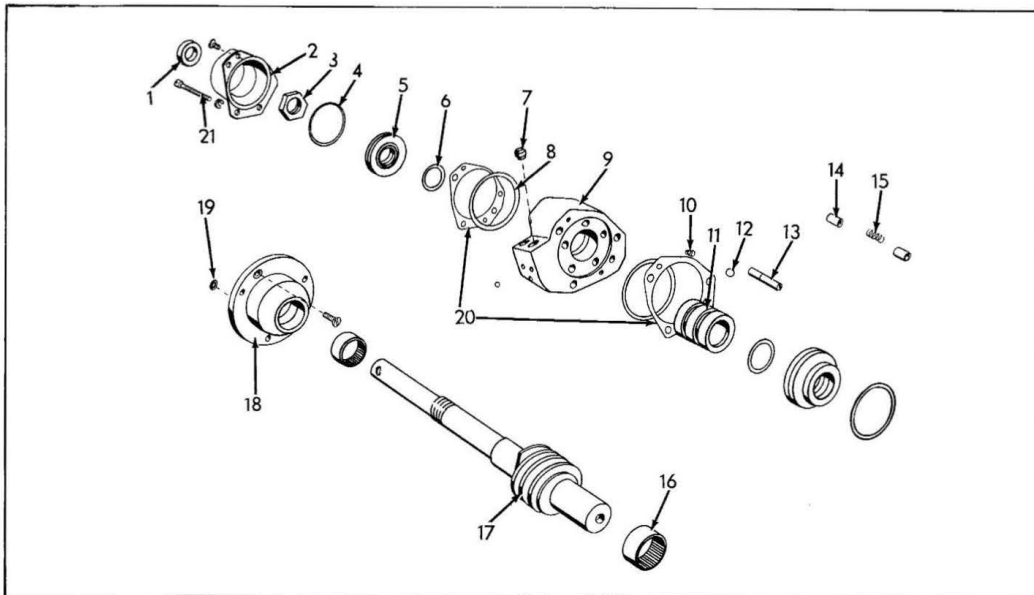
STEERING CONTROL VALVE D-14 Tractor
